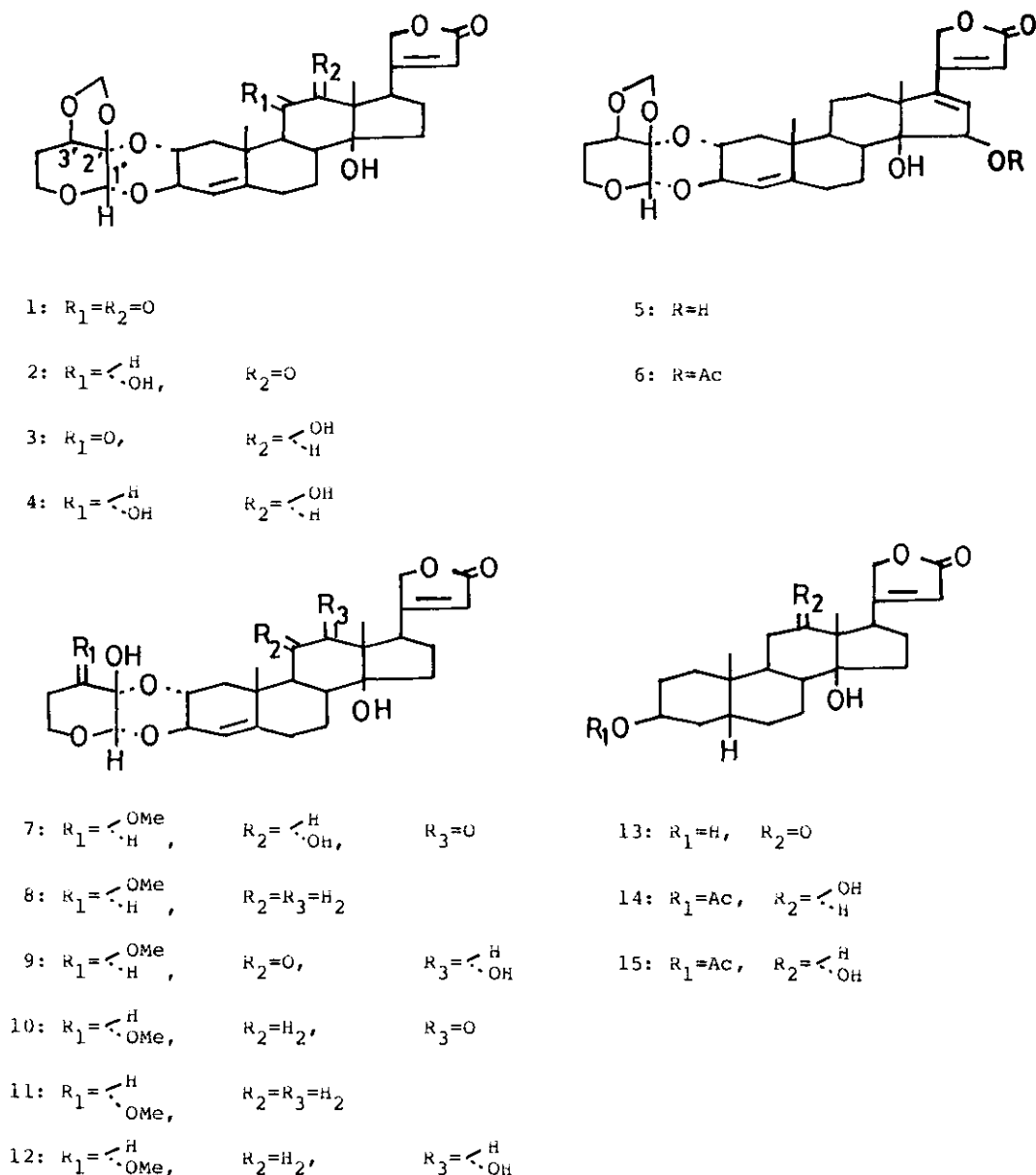
Fig.1. Structures of Elaeodendrosides and Related Compounds
