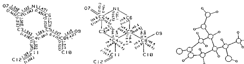
Figure 1. X-ray Structural Analysis of Compound (20a: X=O)
