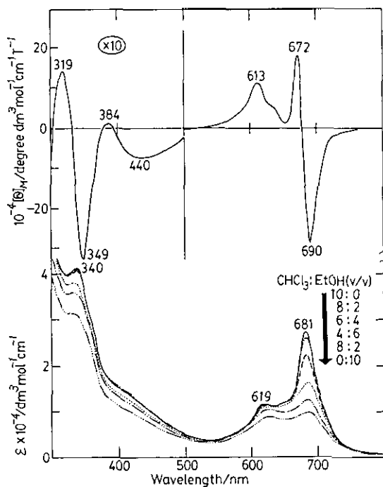
Figure 2. Electronic absorption (bottom) and MCD (top) spectra for \text{Cu}_2\text{CrBPC} in chloroform-ethanol mixtures or in chloroform. [\text{Cu}_2\text{CrBPC}]/\text{M} = 2.78 \times 10^{-5} . Optical path/cm = 1.0. Magnetic field/T = 1.09.
