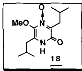
Scheme 3. Synthesis of 2-Hydroxy-3,6-diisobutyl-5-methoxypyrazine 1- and 4-Oxides (14,18).
