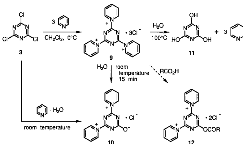
Scheme 4
