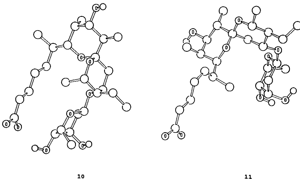
Figure 2: Calculated conformations of 10 and 11 .
