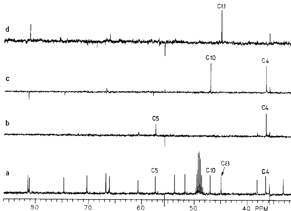
Figure 3. Selective INEPT spectra of 1 in D 2 O (with 3 drops of CD 3 OD). (a) The normal 13 C nmr spectrum for comparison. The quaternary carbons were assigned by the observations of the polarization transfer from (b) H-18, (c) H-2 and (d) H-6.
