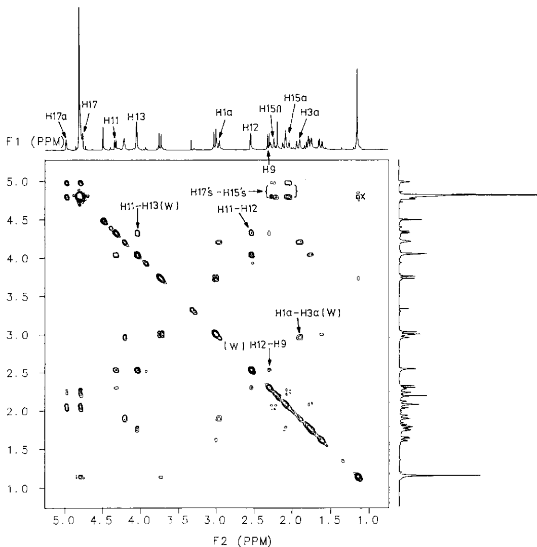
Figure 2. Long range COSY of 1 using a delay of 0.2 s in D 2 O (with 3 drops of CD 3 OD). The capital letter 'W' indicates the important W-couplings. Other labelled peaks are the vicinal coupling between H-11 and H-12 which was not observed in COSY, and the characteristic long range couplings between H-17's and H-15's.
