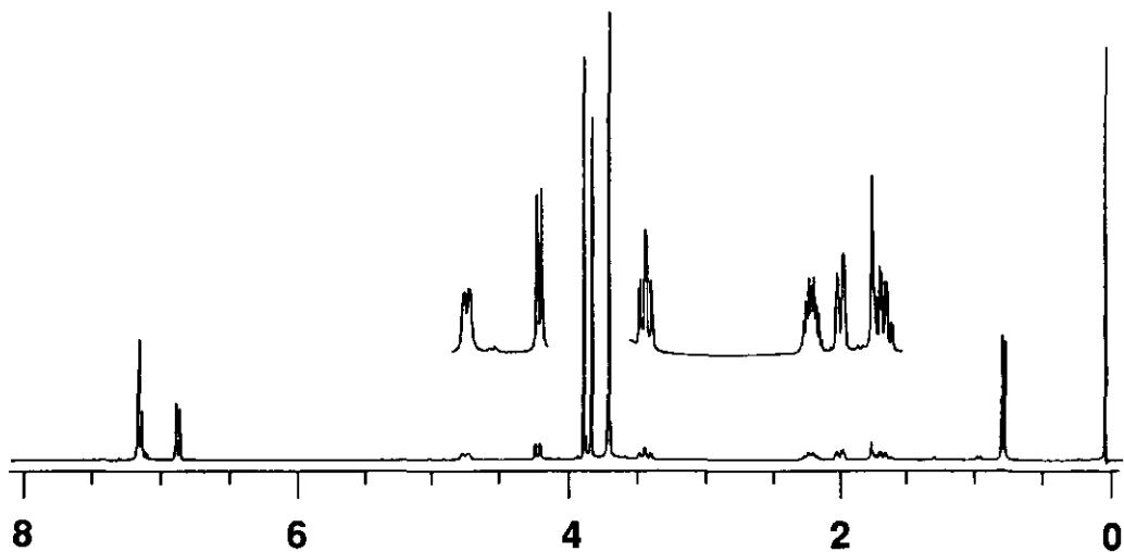
Figure 2. Proton Nmr spectrum of 5-methyl-6-(4-methoxyphenyl)- N -(3,4,5-trimethoxybenzoyl)tetrahydro-1,2-oxazine.
