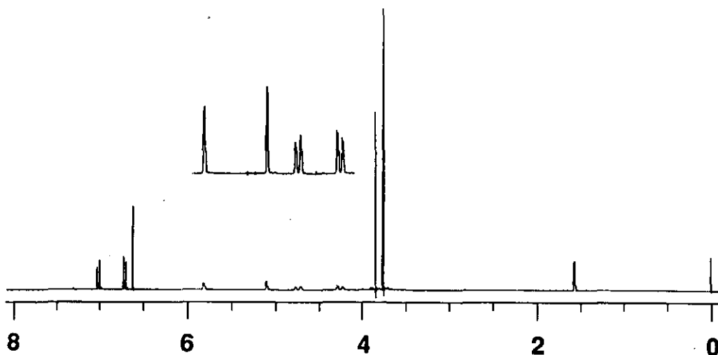
Figure 1. Proton Nmr spectrum of 5-methyl-6-(4-methoxyphenyl)-3,6-dihydro-1,2-oxazine
