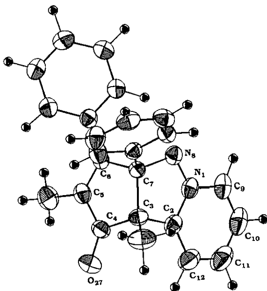
Figure 1. Structure of 1a: Selected bond lengths ( \text{\AA} ): N1-C2 1.372(3); N1-C9 1.372(3); C9-C10 1.373(5); C10-C11 1.390 (5); C11-C12 1.375(3); C12-C2 1.378(4); C2-C3 1.498(3); C3-C7 1.577(4); C7-N8 1.481(2); N1-N8 1.337(3)
