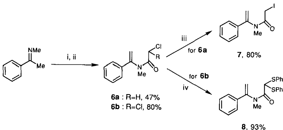
Scheme 1. Reagents and conditions: i, \text{RCICHCOCl} (R=H or Cl), \text{CH}_2\text{Cl}_2 ; ii, sat. \text{NaHCO}_3 ; iii, NaI, MeCN; iv, \text{PhSNa} (2.2 equiv.), EtOH.
