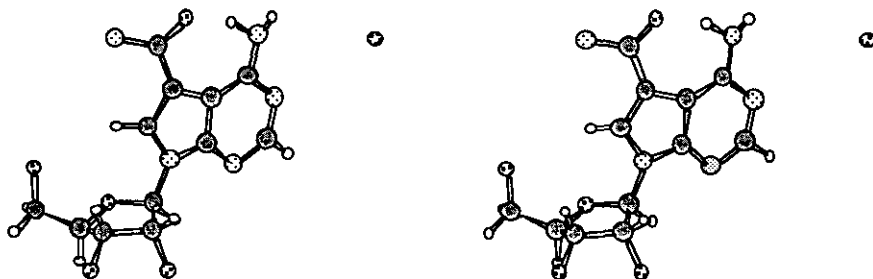
Figure 4 Sangivamycin ( 1 )
