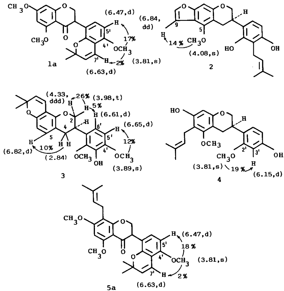
Figure 3 NOE values for 1a, 2, 3, 4, and 5a, measured in acetone- d_6 (1a, 4, and 5a) and CDCl_3 (2 and 3)
