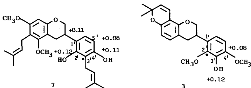
Figure 4 Deuterium induced isotope shift ^{13}\text{C} nmr experiments of 7 and 3. Each 5 mg of samples were measured in 0.6 ml of acetone- \text{d}_6 , added one drop of the mixture of \text{D}_2\text{O} and \text{H}_2\text{O} in 1:1. * These carbon signals were observed as broad singlet.
