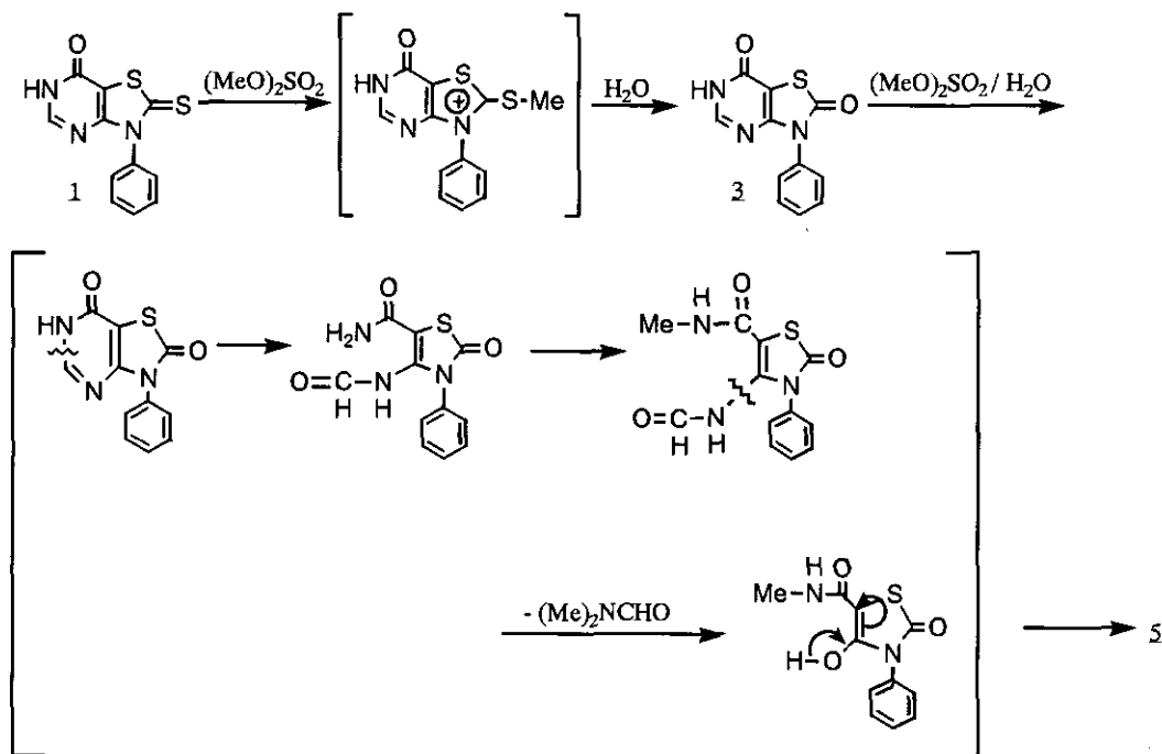
Scheme 3
