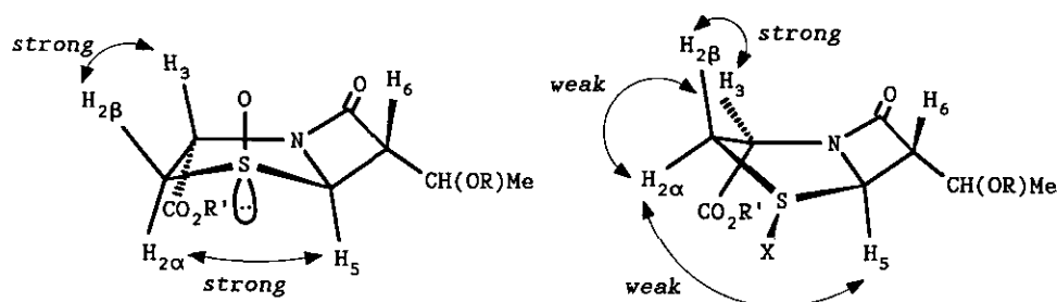
Figure 1. Possible thiazolidine ring conformations: open or pseudoequatorial (left), and closed or pseudoaxial (right). Arrows indicate relevant NOEs observed for 10 (left) and for 1a, 11 (right; X= lone pair or O, respectively).
