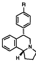
1 R = H 2 R = SMe
