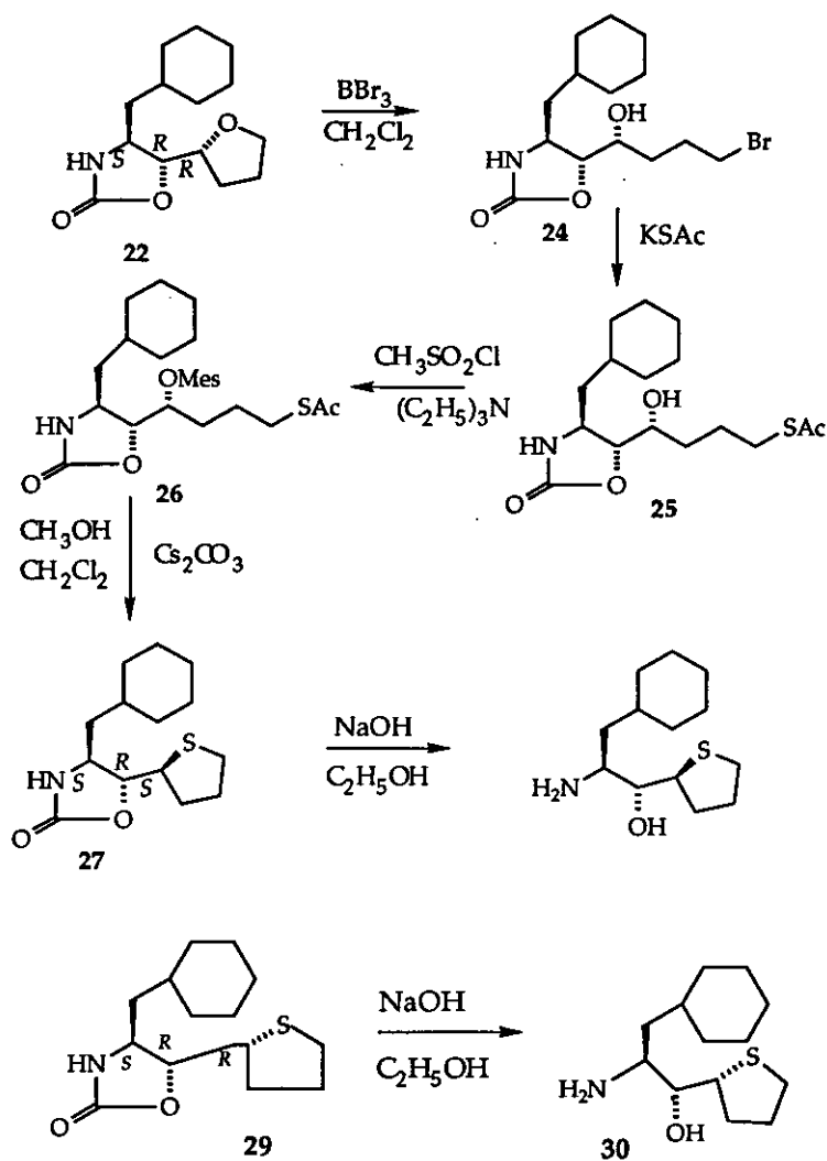
Scheme III
