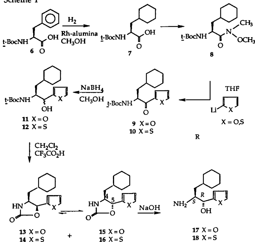
Scheme I
