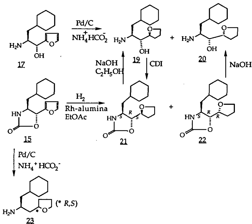
Scheme II
