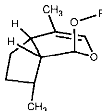
Figure 2. Conformation of 3 (R=ethoxyethyl)
