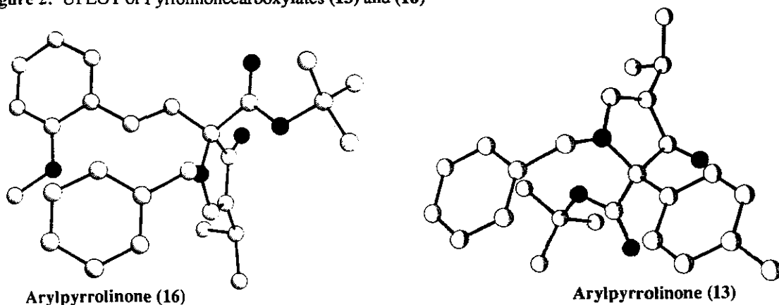
Figure 2: UPLOT of Pyrrolinonecarboxylates (13) and (16)
