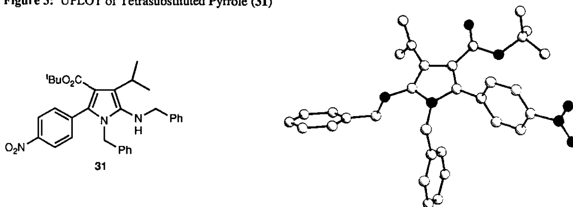
Figure 3: UPLOT of Tetrasubstituted Pyrrole ( 31 )
