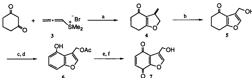
Scheme I. Reagents and Conditions ; (a) NaOEt, EtOH, room temperature, 50%. (b) MMPP, Bu 4 Nl, CH 2 Cl 2 / H 2 O, 0 °C, 78%. (c) Ac 2 O, Pyridine, DMAP, 0 °C, 99%. (d) TBDMSOTf, NEt 3 , 0 °C, then Pd(OAc) 2 , 48%. (e) K 2 CO 3 , MeOH, 0 °C, 92%. (f) Fremy's salt, H 2 O-KH 2 PO 4 buffer, 0 °C, 69%.
