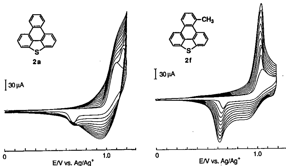
Figure 1. The Cyclic Voltammograms of Compounds (2a) and (2f) with Repeated Scan in CH 3 CN (0.1 M NaClO 4 ); 2a (2.0 mM), 12 Times; 2f (0.9 mM), 10 Times.
