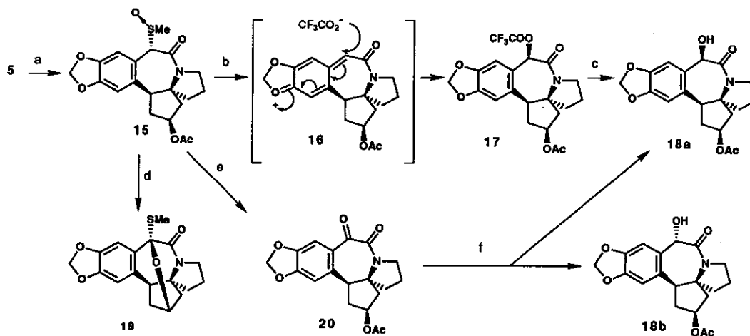
Scheme 2. Reagents and conditions: (a) MCPBA, \text{CH}_2\text{Cl}_2 ; (b) (\text{CF}_3\text{CO})_2\text{O} , \text{CH}_2\text{Cl}_2 ; (c) silica gel; (d) TsOH \text{H}_2\text{O} , (\text{CH}_2\text{Cl}_2)_2 , reflux; (e) TsOH, (\text{CH}_2\text{Cl}_2)_2 , reflux; (f) \text{NaBH}_4 , EtOH at -20°C
