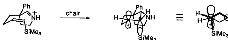
Figure 1. Optimal overlap of the \beta -C-Si \sigma -bond and the developing cyclohexyl cation in a chair topography cyclization of a ( Z )-vinylsilane.
