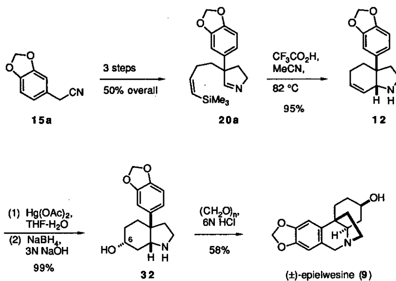
Scheme 4. Total Synthesis of (±)-Epielwesine
