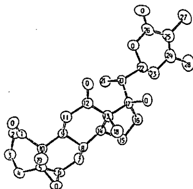
Figure 1. Perspective drawing of (-)-jaboromagellonine (1).
