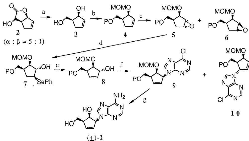
Scheme 2. P = SiPh 2 - t -Bu. Reagents and conditions: a, i, LiAlH 4 , Et 2 O, ii, NaIO 4 , CH 2 Cl 2 -H 2 O, iii, NaBH 4 , MeOH, 54%; b, i, t -BDPSCI, NEt 3 , DMAP, CH 2 Cl 2 , ii, MOMCl, i -Pr 2 NEt 3 , CH 2 Cl 2 , 81%; c, m -CPBA, CH 2 Cl 2 , 94%; d, PhSeSePh, NaBH 4 , n -BuOH, reflux, 2 h; e, 30% H 2 O 2 , THF, 70% from 5 ; f, 6-chloropurine, Ph 3 P, DEAD, THF, -40 °C \rightarrow room temperature, 10%; g, i, Bu 4 NF, THF, ii, NH 3 , MeOH, 80 °C (sealed tube), iii, conc. HCl, MeOH, reflux, 1 h, 64%.
