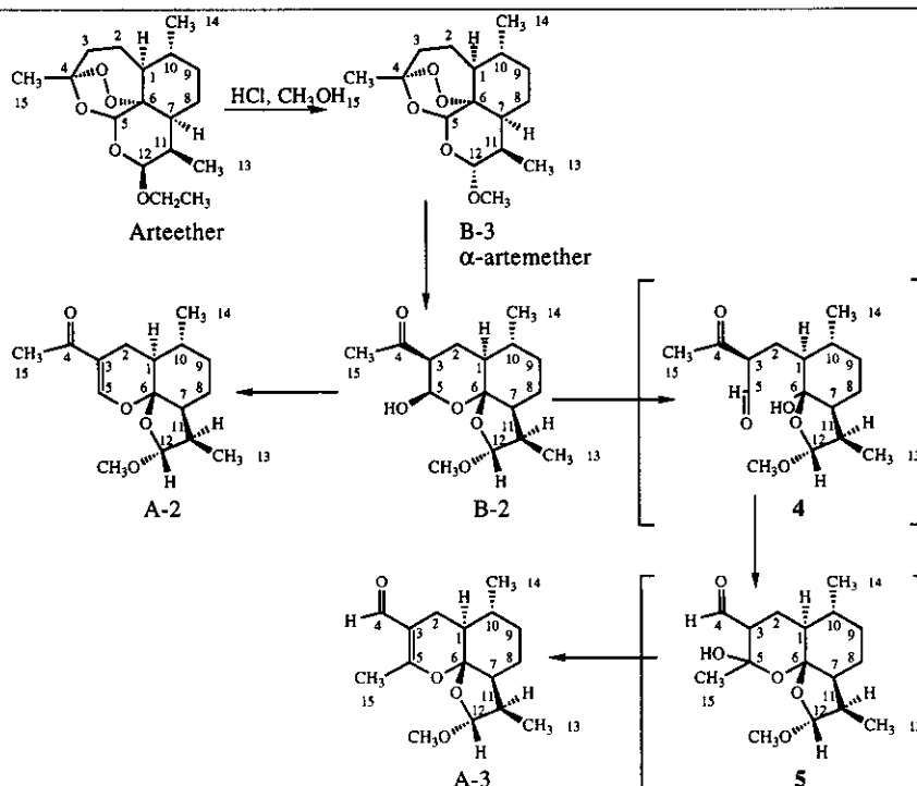
Figure 4: Proposed mechanism for the formation of the A- and B-series of Arteether products
