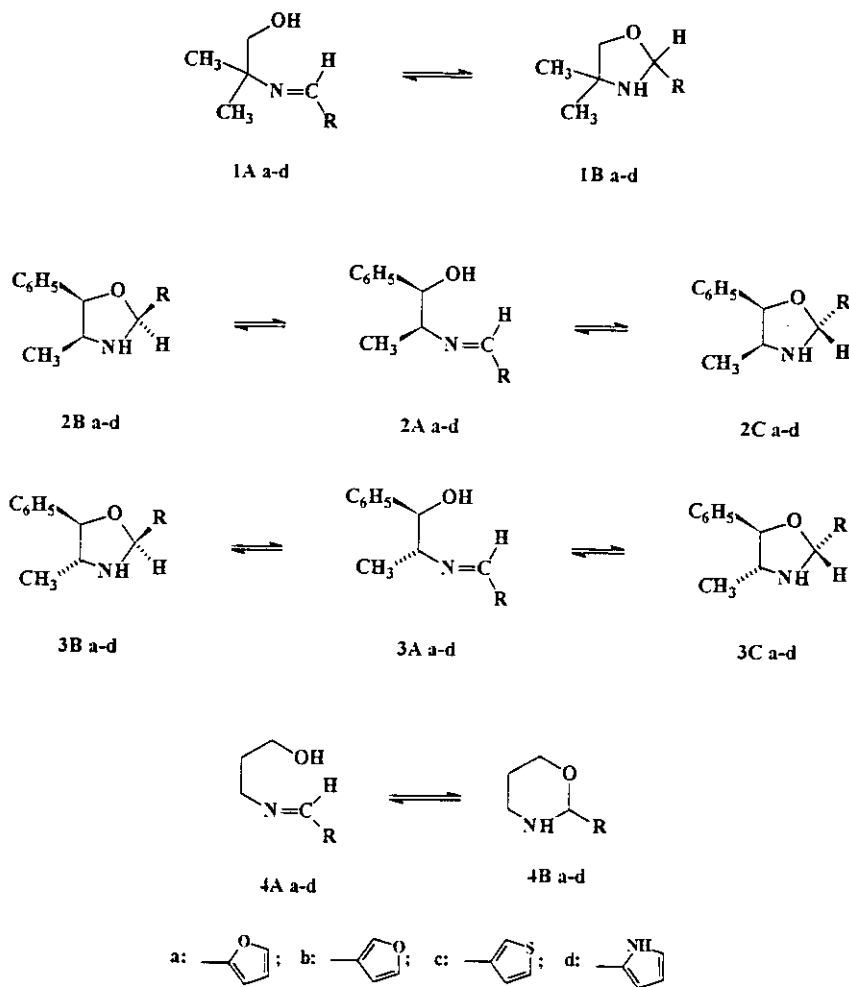
Scheme 1
