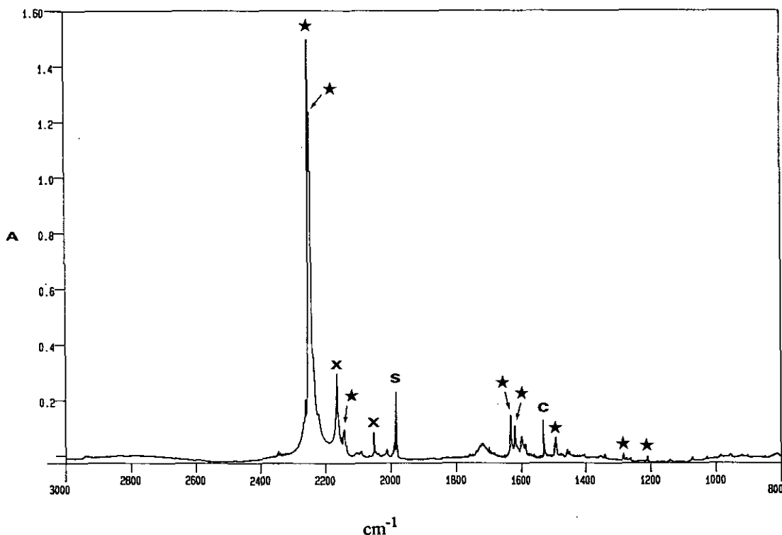
Figure 1: FTir spectrum (Ar matrix, 18 K) of the FVP of 1b ( 900^\circ\text{C} , 5 \times 10^{-5} mbar). \text{Ph-NC}_3\text{O} (★) appears at 2247\text{vs} , 2243\text{vs} , 2141\text{w} , 1661\text{m} , 1620\text{m} , 1490\text{w} , 1284\text{w} , and 1210\text{w cm}^{-1} . Other bands are due to \text{HNCS} (S, 1981\text{ cm}^{-1} ), \text{CS}_2 (C, 1528\text{ cm}^{-1} ), and unidentified by-products (X, 2163 , 2049\text{ cm}^{-1} ).
