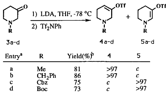
Scheme 1. The Synthesis of Triflates
