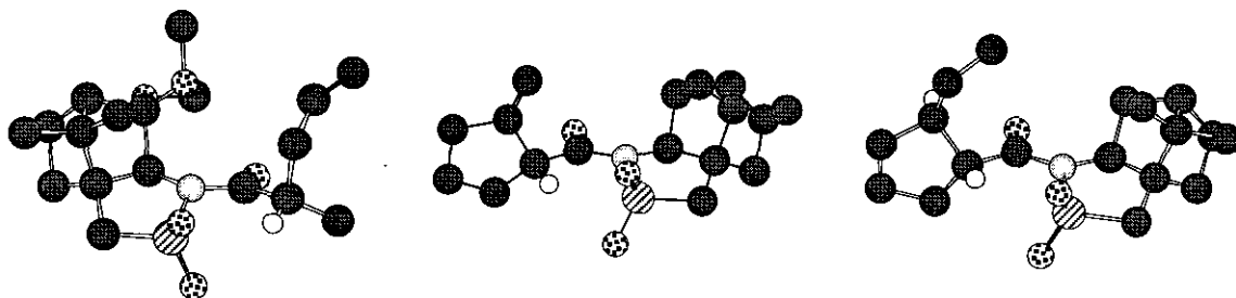
Figure 2. Crystal Structures of 9a (left), 19 (center) and 25b (right)
