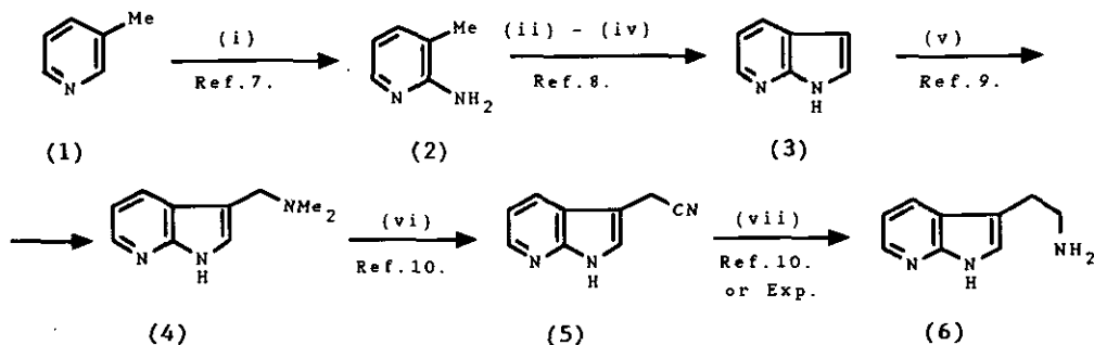
Scheme 1 Preparation of 7-azatryptamine
