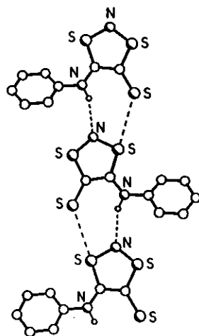
Figure 3 Part of one of the hydrogen-bonded chains of molecules in the crystal of 18
