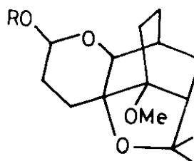
17 (a) R = Me
