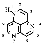
1 H -1,4,7-Triazaphenalene
