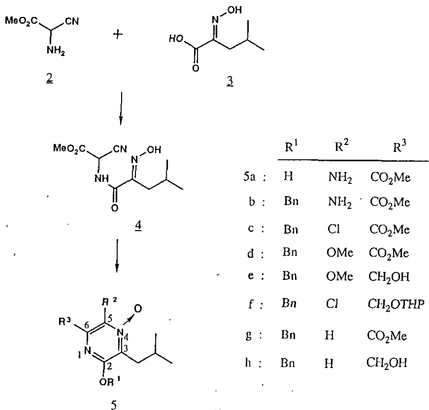
Scheme Synthetic pathway of pyrazine 4-oxide derivatives (5)
