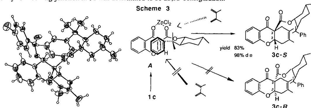
Figure 1. ORTEP drawing of 6
