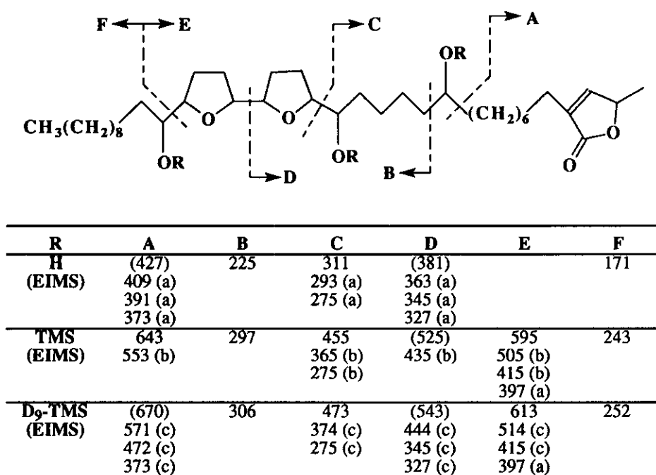
Figure 2. Diagnostic EIms fragmentation ions of 2 and its tri-TMS and tri-d 9 -TMS derivatives
