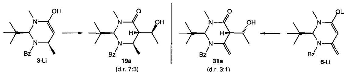
Scheme 20
