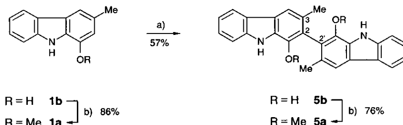
Scheme 2: The dimerization to biscarbazole derivatives. Reagents and conditions: a) (t\text{-BuO})_2 , chlorobenzene, reflux, 3 h; b) \text{CH}_2\text{N}_2 / \text{Et}_2\text{O} , MeOH, 5 °C, 12 h (for 1b ), resp. 24 h (for 5b ).
