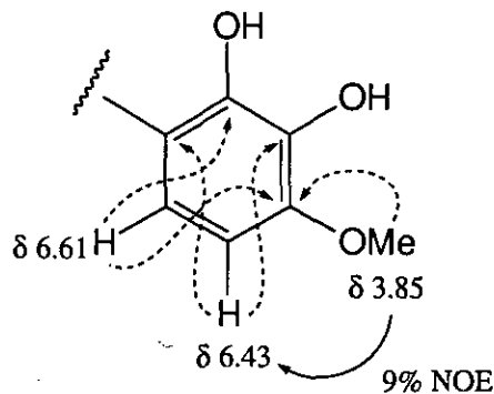
Figure 1 ^3J Interaction Observed in the Long-Range CH COSY of 5b (-----) and NOE
