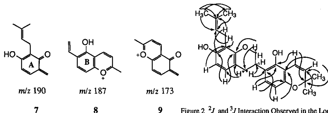
Figure 2 ^2J and ^3J Interaction Observed in the Long-Range CH COSY of 8-Prenyl-phaseollinisoflavan
