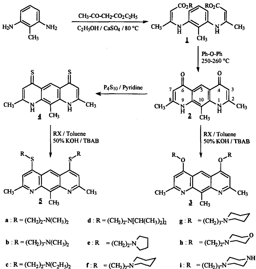
Scheme 1
