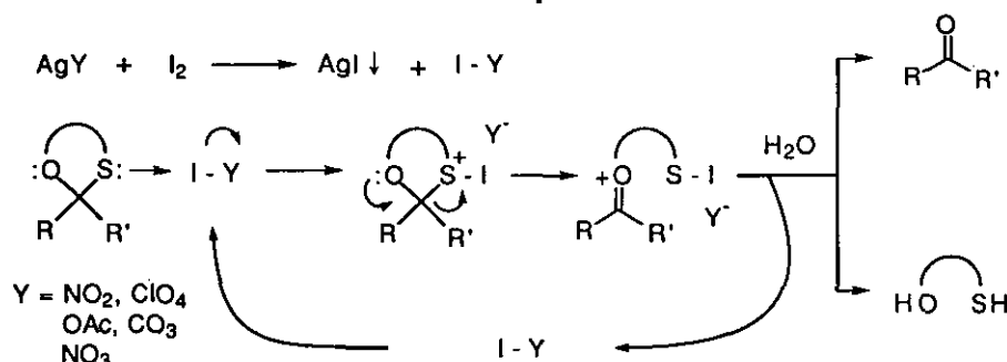
Scheme 1. A Possible Mechanism for Deprotection
