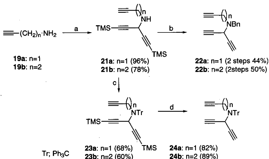
Scheme 5 a
