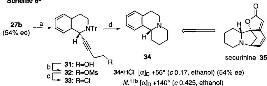
Scheme 8 a
