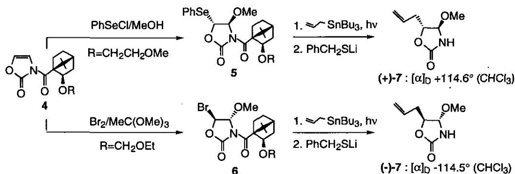
Scheme 1 7
