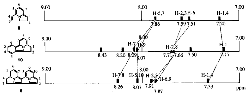
Figure 1. ^1\text{H} -NMR spectra of 8, 9, and 10
