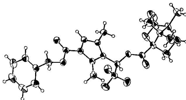
Figure 1 X-ray analysis of ( S )- 5
