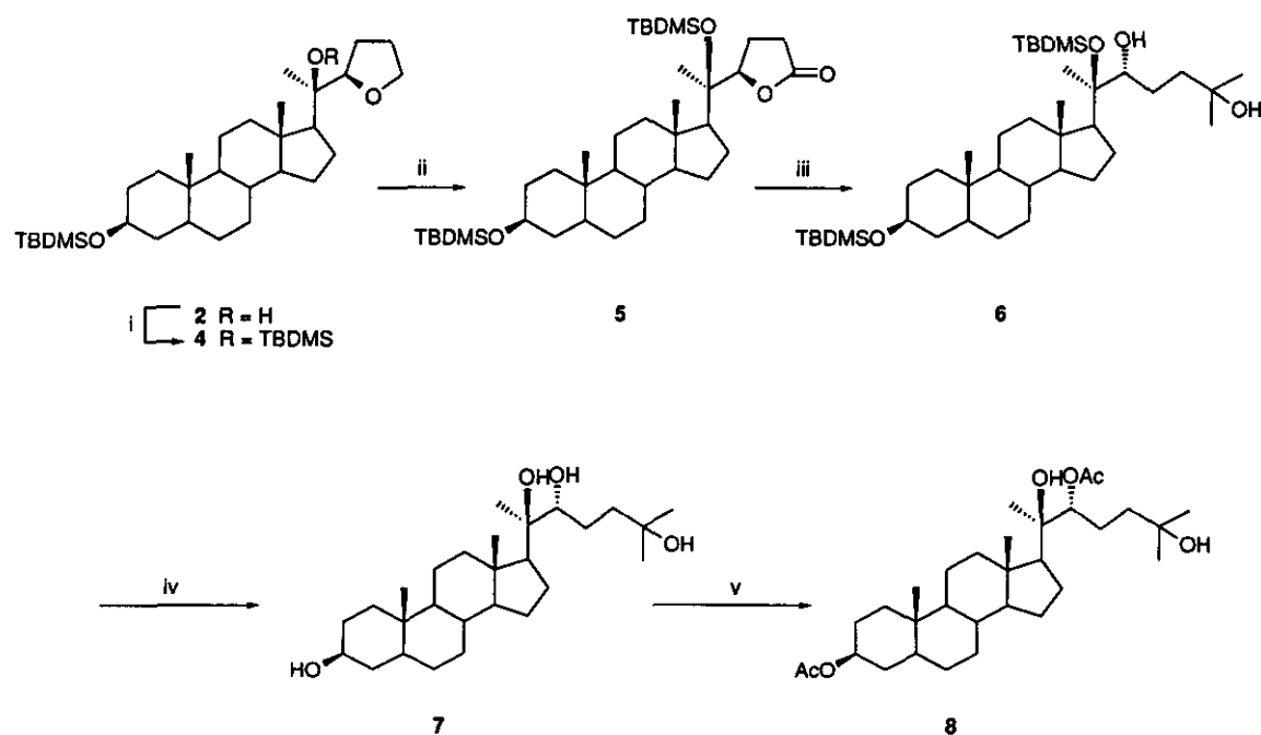
Scheme 2. Reactions and conditions: i, TBDMSOTf, 2,6-lutidine, \text{CH}_2\text{Cl}_2 , rt; ii, \text{RuO}_2 , \text{NaIO}_4 , \text{CCl}_4 - \text{MeCN} - \text{H}_2\text{O} , rt; iii, \text{MeMgBr} , THF, -78^\circ\text{C} ; iv, TBAF, THF, rt; v, \text{Ac}_2\text{O} , pyridine, rt.
