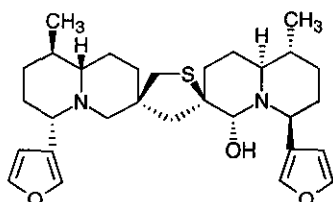
6-hydroxythionuphlutine B (7)
