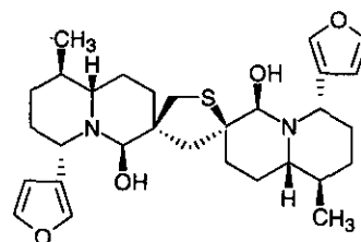
6,6'-dihydroxythiobinupharidine (6)
