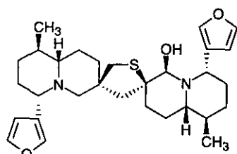
6-hydroxythiobinupharidine (5)
