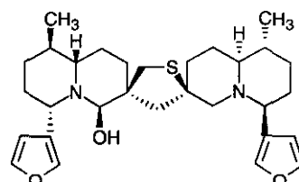
6'-hydroxythionuphlutine B (8)
