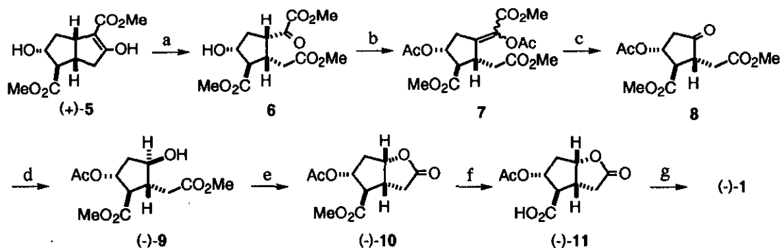
Scheme 2. A Facile Asymmetric Synthesis of Corey Lactone
