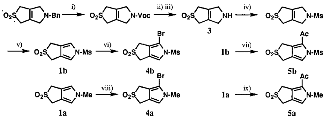
Scheme 2 Reagents and conditions: i, Voc-Cl, 1,2-dichloroethane, 0 °C; ii, \text{Br}_2 , dichloromethane, -15 °C; iii, MeOH, 50 °C; iv, Ms-Cl, pyridine, 0 °C, 71.3%; v, chemical \text{MnO}_2 (40 mol-equiv.), dichloromethane, rt, 80.6%; vi, NBS (3.3 mol-equiv.), THF, rt, 76.8%; vii, \text{Ac}_2\text{O} (2.2 mol-equiv.), \text{BF}_3 \cdot \text{Et}_2\text{O} (4.4 mol-equiv.), 1,2-dichloroethane, rt; viii, NBS (0.9 mol-equiv.), THF, -78 °C; ix, \text{Ac}_2\text{O} (1.1 mol-equiv.), \text{BF}_3 \cdot \text{Et}_2\text{O} (2.2 mol-equiv.), 1,2-dichloroethane, rt.
