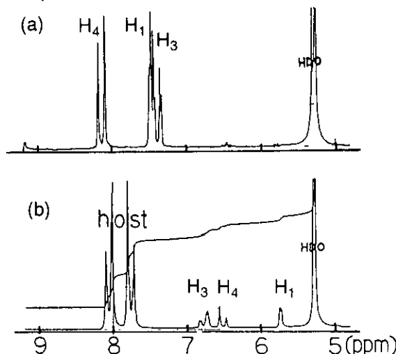
Figure 2. 1 H NMR spectra of (a) guest (9) and (b) TCP44 (2) + guest (9) in DCl-D 2 O (pD 1.2) [2] = 5.0 \times 10^{-2} M, [9] = 2.5 \times 10^{-2} M. TMS as an external reference.
